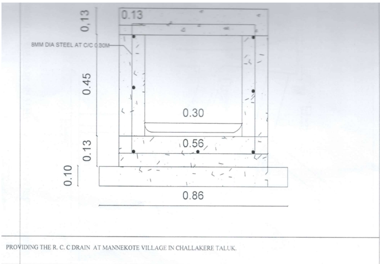
Drain Section
